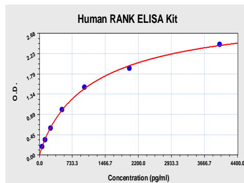
Figure 1: RANK Standard Curve. Using the Human RANK ELISA Kit, O.D. data was graphed against RANK protein concentration. The TMB reaction was incubated at 37°C for 23 min.
